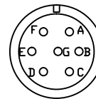
MS3102A24-10P Motor Cable Connector 접속도
