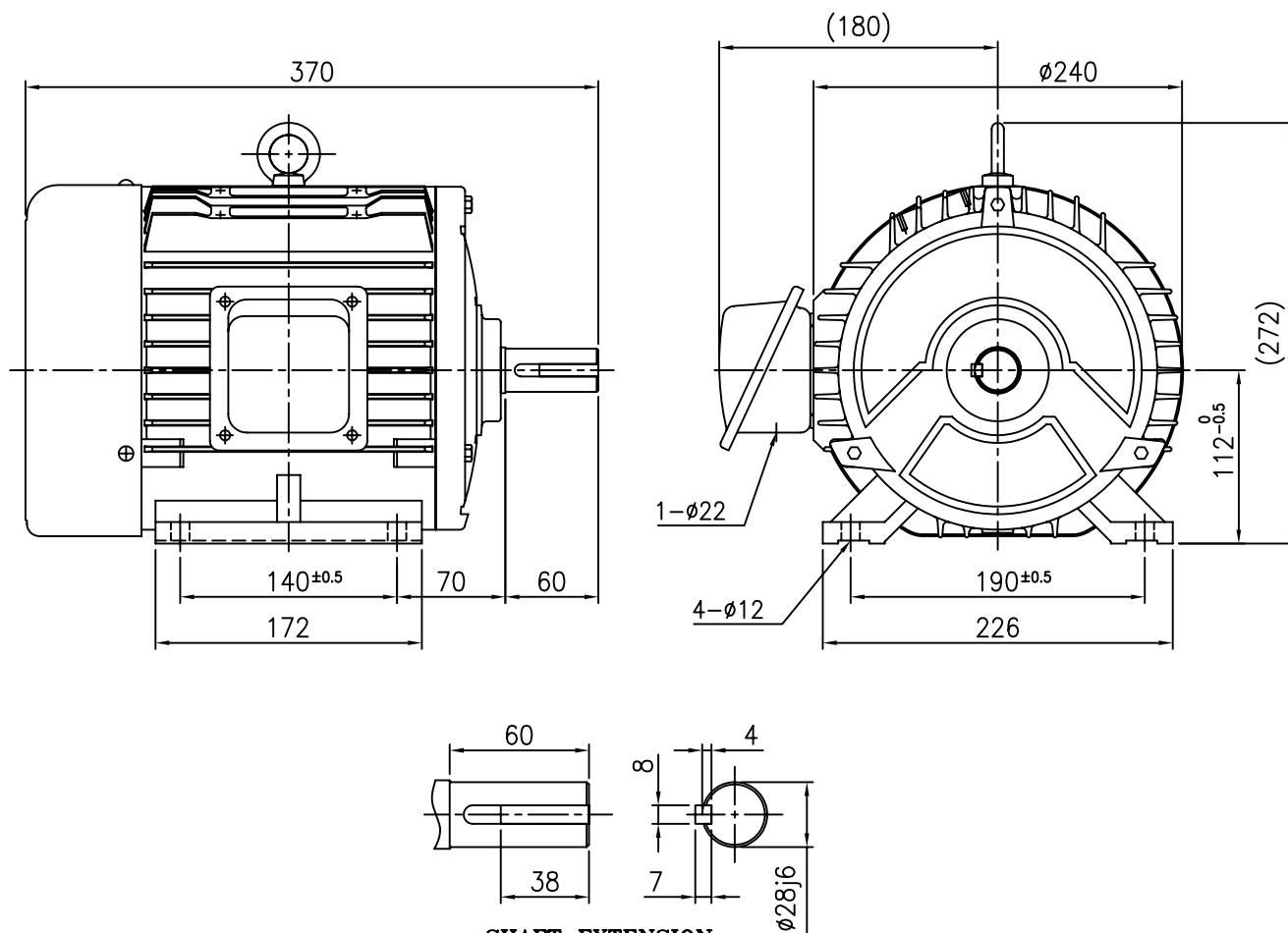
SHAFT EXTENSION
