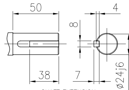
SHAFT EXTENSION
