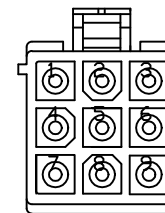
AMP 172169-1 PLUG 9P AMP 170359-1 PIN
