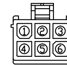
AMP 172168-1 Plug 170360-1 PIN
