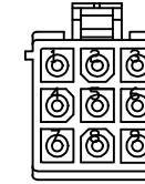
AMP 172169-1 PLUG 9P AMP 170359-1 PIN
