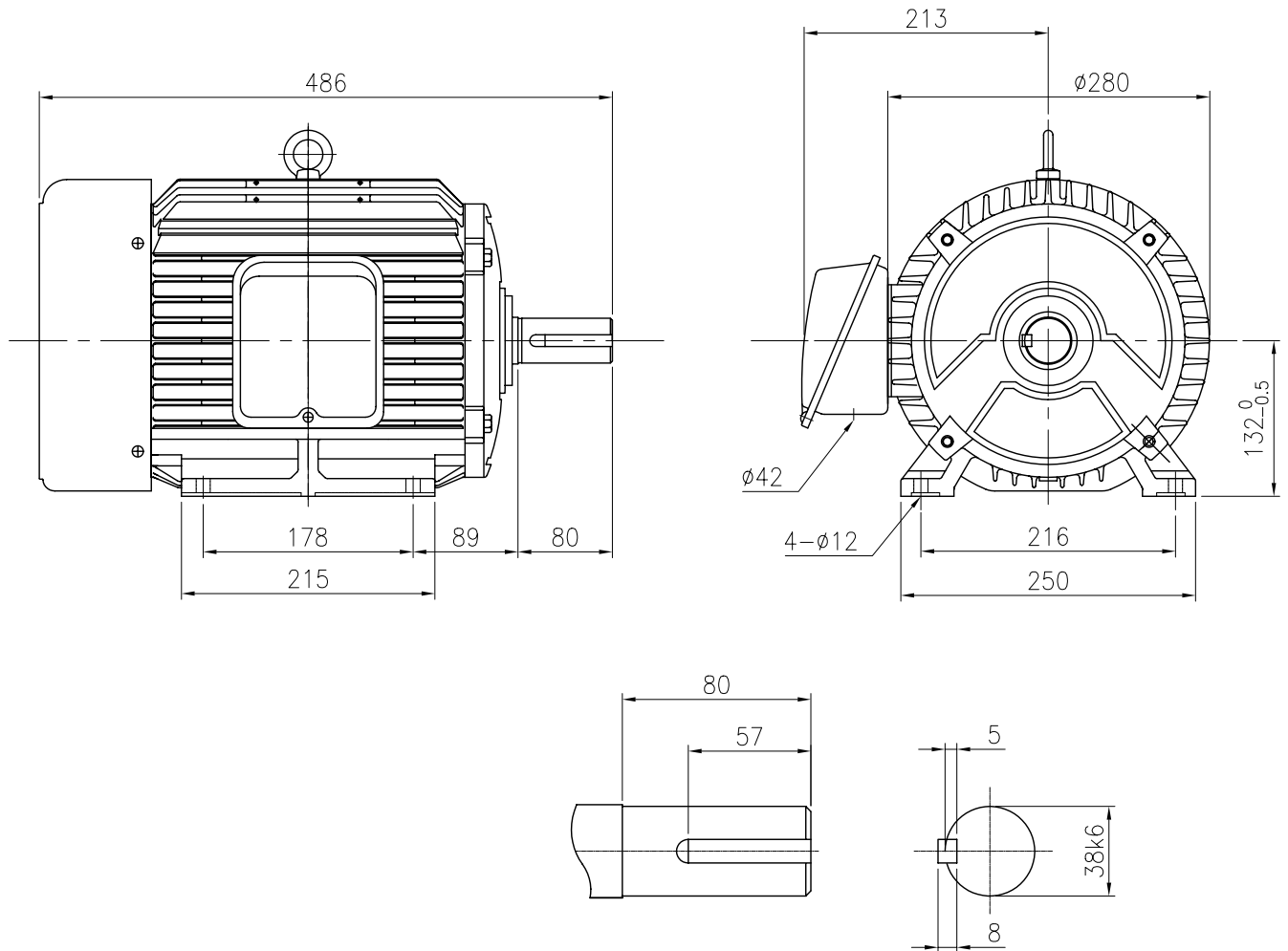
SHAFT EXTENSION
